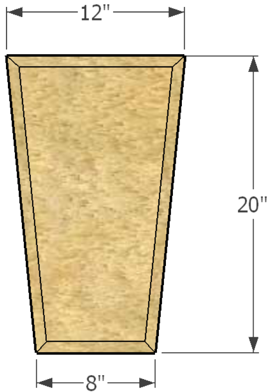
A 1 Product#8-01P Front View
