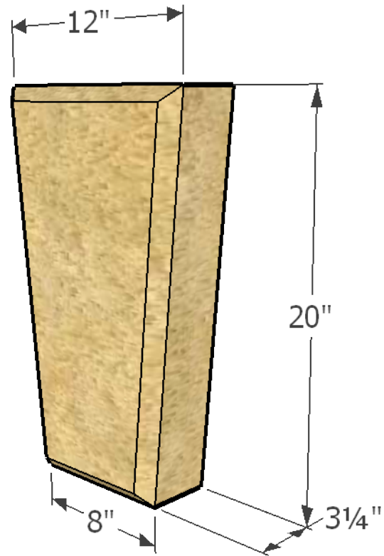
A 1 20" Beveled Perspective
